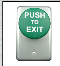
SMPX60 1 switch SPDT momentary, 2-3/8" (60mm) Green Button, "PUSH TO EXIT" Button ICON with White Letters, Plain Faceplate with BHMA 689 finish.
